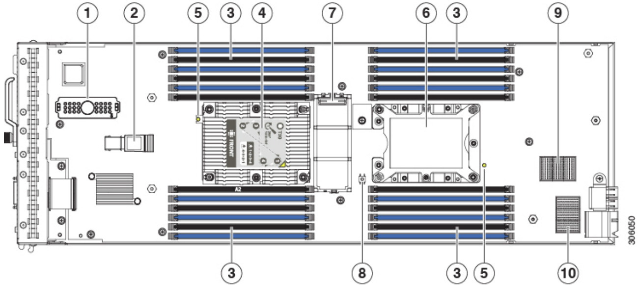
Figure 5 UCS B200 M5 System Board
