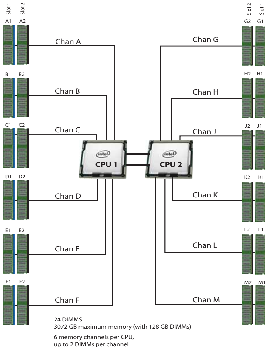
Figure 4 C220 M5 LFF Memory Organization
