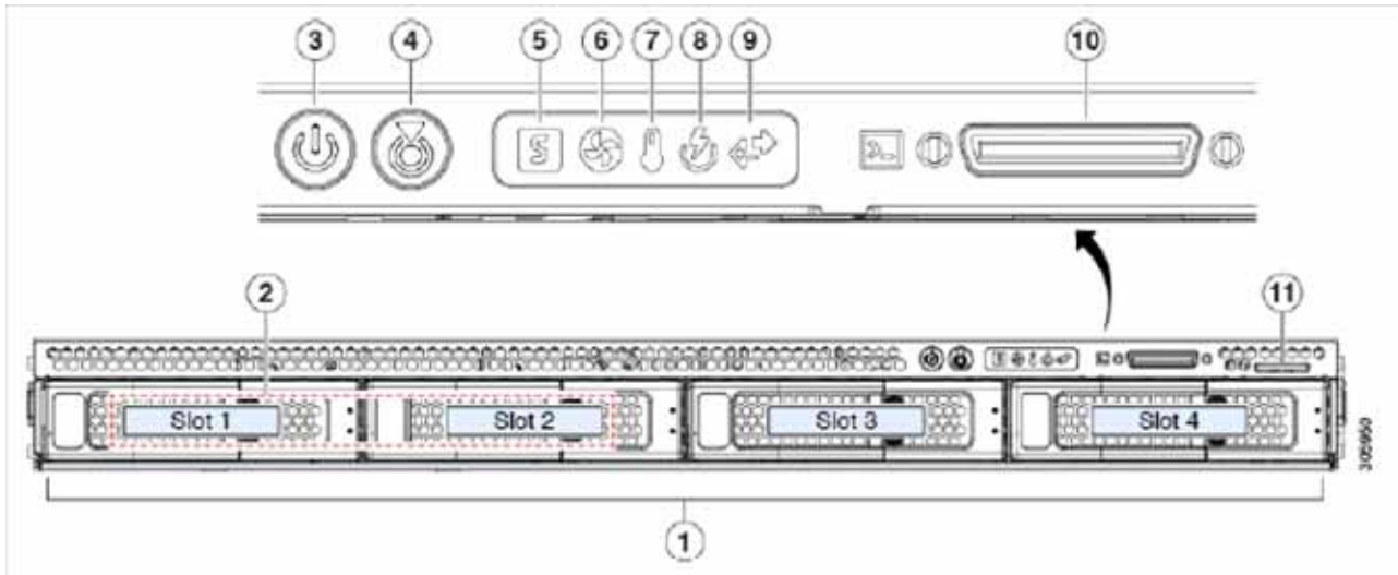
Figure 2 Chassis Front View
