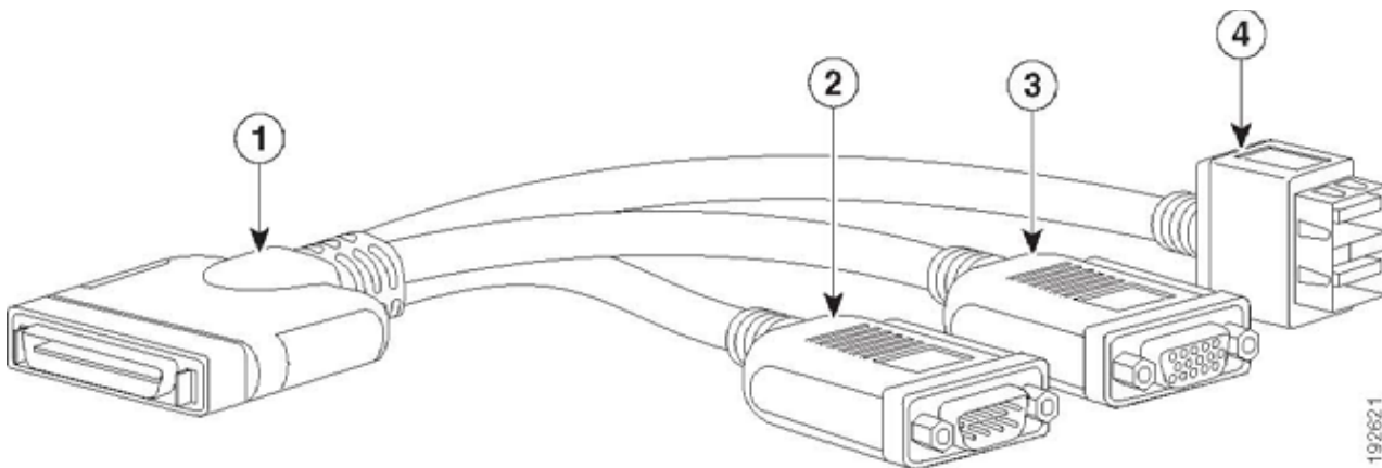
Figure 9 KVM Cable
